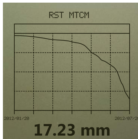
A close-up of the display on the MTCM - Graphing Logger showing a typical reading with graph.
