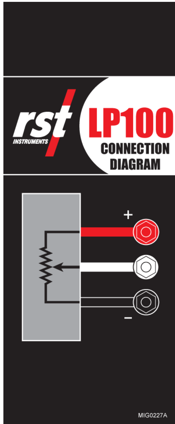
Figure 2 – Wiring Connections
