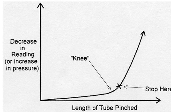
Figure 5 – Cell Re-Pressurization Graph
