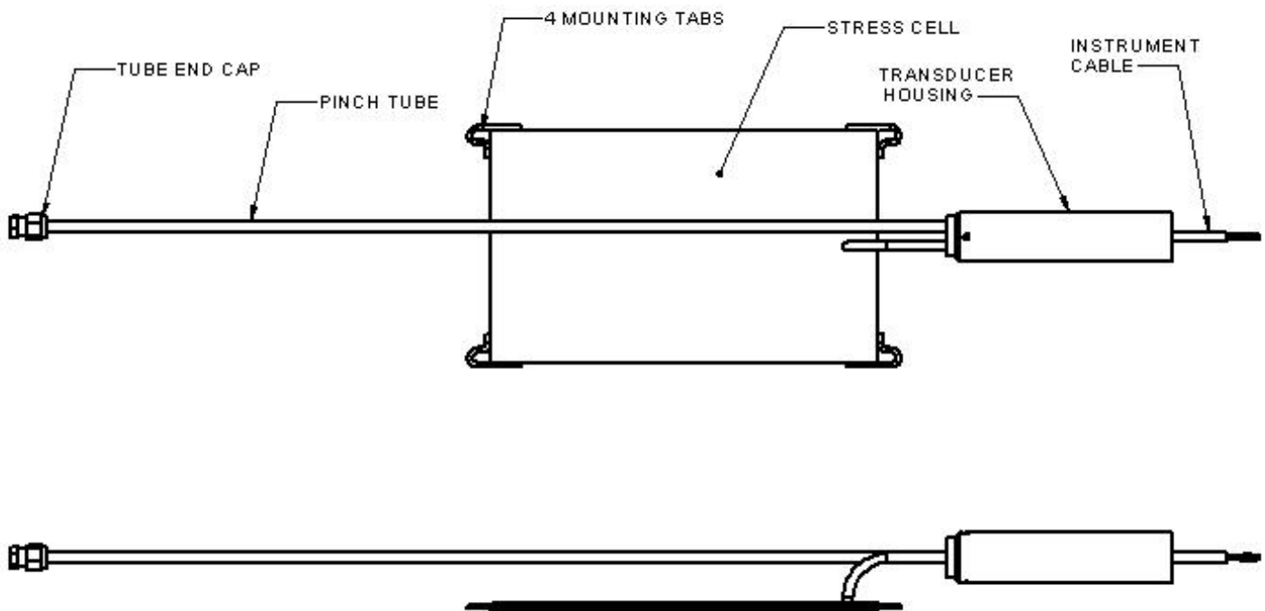
Figure 2 Concrete Stress Cell GA
