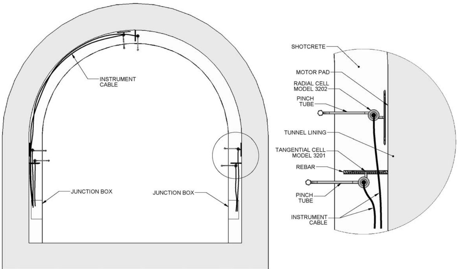
Figure 4 –Post Shotcrete General Arrangement
