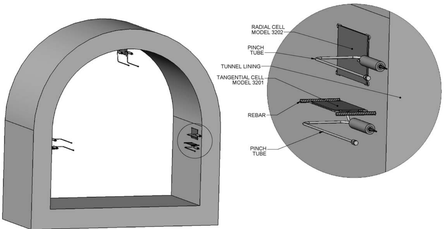
Figure 3 – General Arrangement
